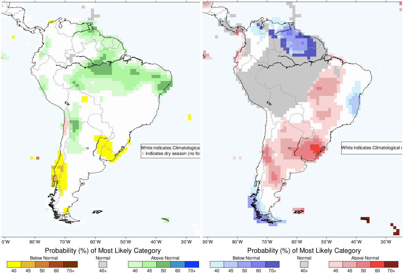
IRI Multi-Model Probability Forecast for Precipitation for February-March-April 2023, Issued January 2023
