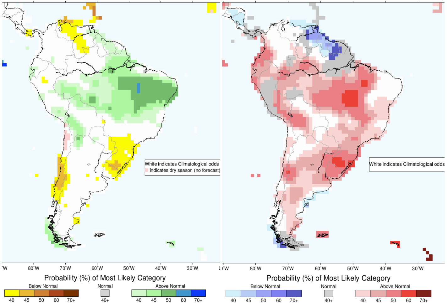
IRI Multi-Model Probability Forecast for Precipitation for March-April-May 2023, Issued February 2023
