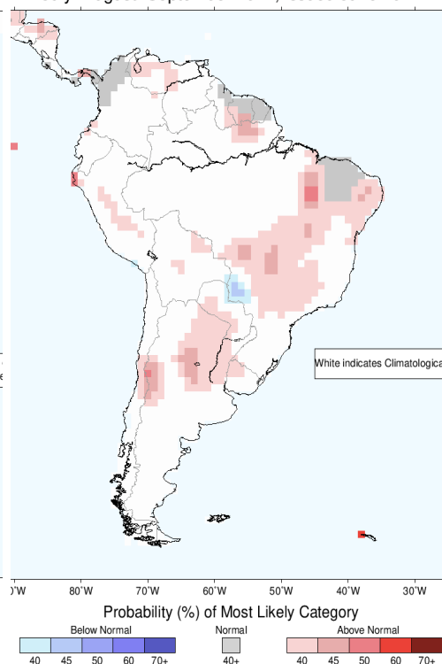
IRI Multi-Model Probability Forecast for Temperature for July-August-September 2021, Issued June 2021
