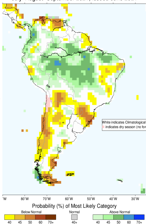
IRI Multi-Model Probability Forecast for Precipitation for July-August-September 2021, Issued June 2021
