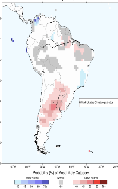
IRI Multi-Model Probability Forecast for Temperature for November-December-January 2021, Issued October 2020
