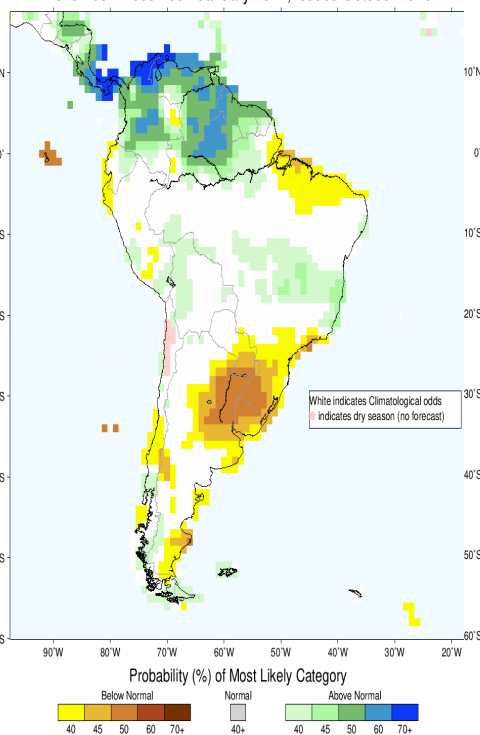
IRI Multi-Model Probability Forecast for Precipitation for November-December-January 2021, Issued October 2020
