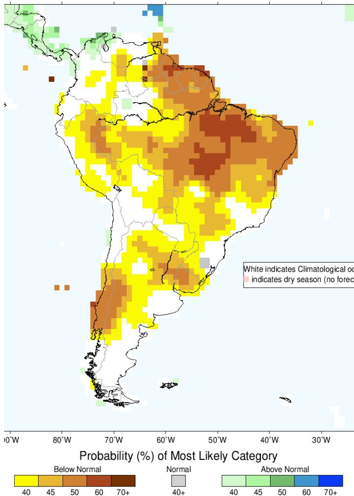
IRI Multi-Model Probability Forecast for Precipitation for September-October-November 2024, Issued August 2024
