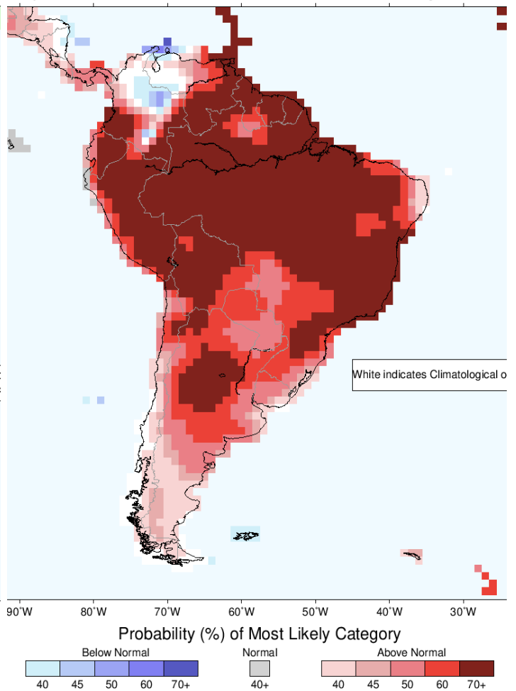
IRI Multi-Model Probability Forecast for Temperature for September-October-November 2024, Issued August 2024
