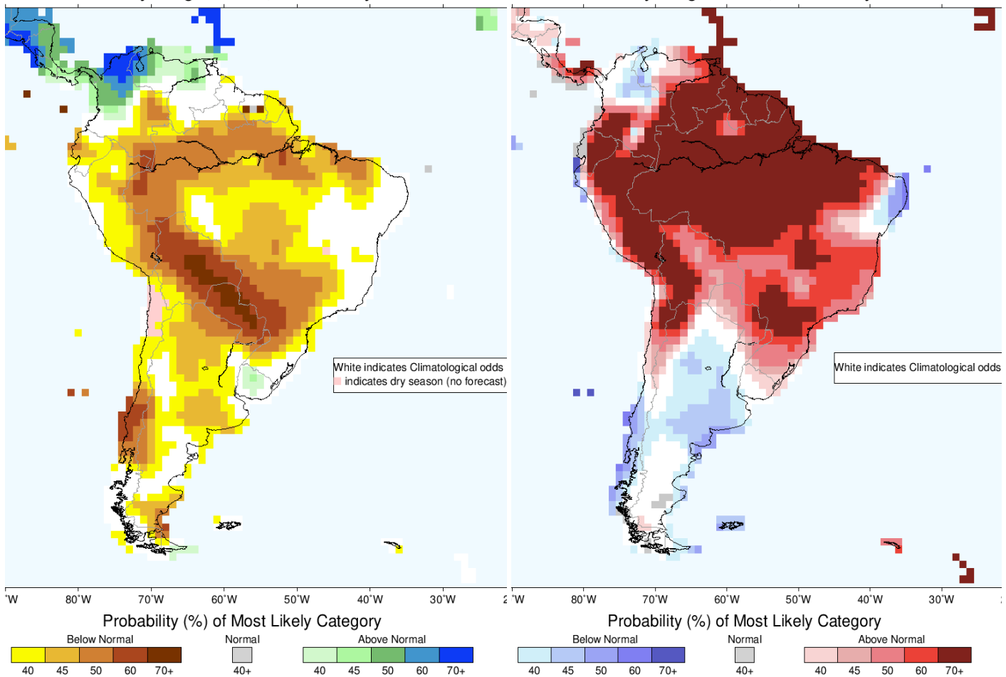
IRI Multi-Model Probability Forecast for Precipitation for June–July–August 2024, Issued May 2024
