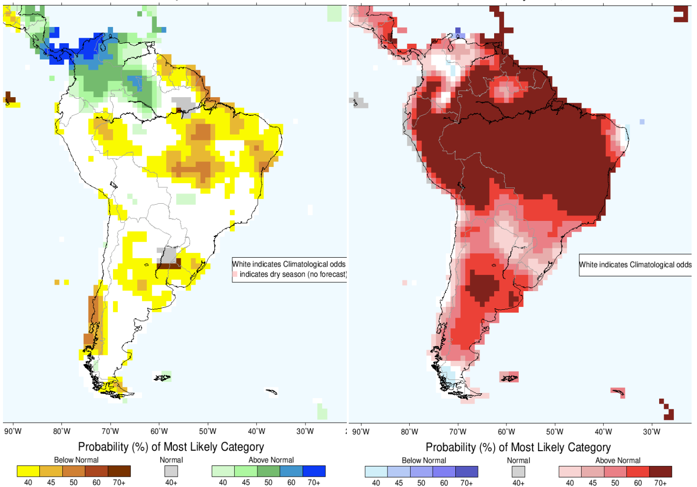
IRI Multi-Model Probability Forecast for Precipitation for November-December-January 2025, Issued October 2024
