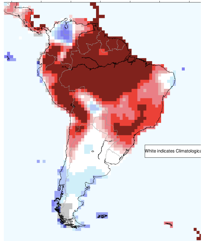
IRI Multi-Model Probability Forecast for Temperature for May-June-July 2024, Issued April 2024
