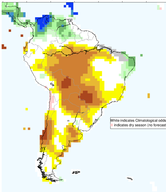
IRI Multi-Model Probability Forecast for Precipitation for May-June-July 2024, Issued April 2024
